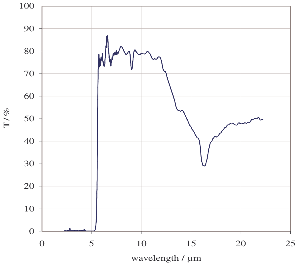
Typical Transmission 5.5 \mu m Filter
